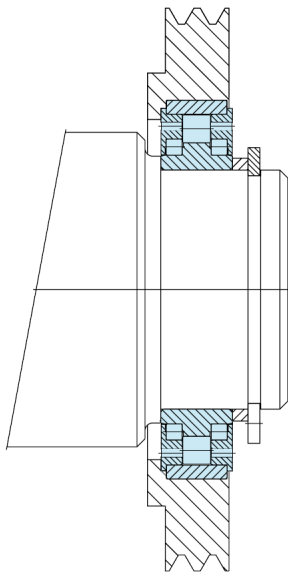
Fig. 3 Mounting ASK
